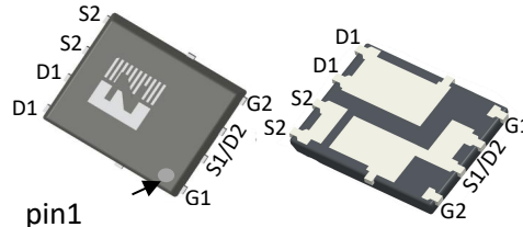
DFN5*6
